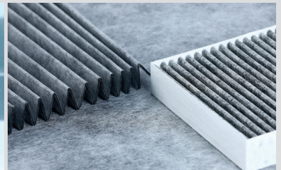
Flat Filter Media Flachfiltermedien
