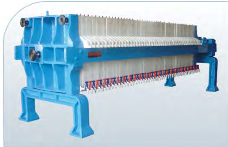
Widened leg cast iron Filter Press
