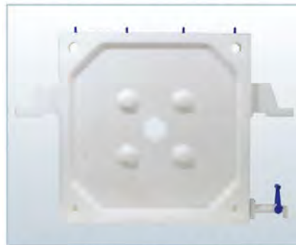
Four port Recess Chamber Filter Plate with integrated Handle
