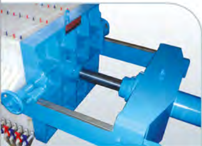
Double acting pull back type Hydraulic Cylinder coupled with moving head
