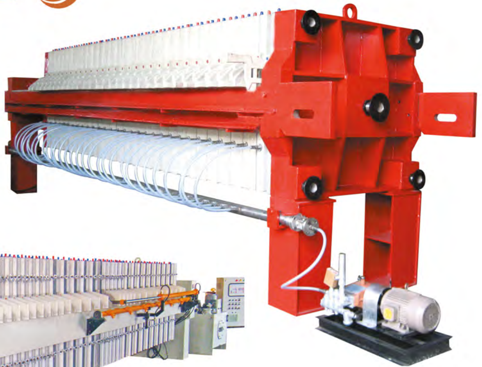
Automatic Filter Press with Polypropylene Membrane type filter plates
